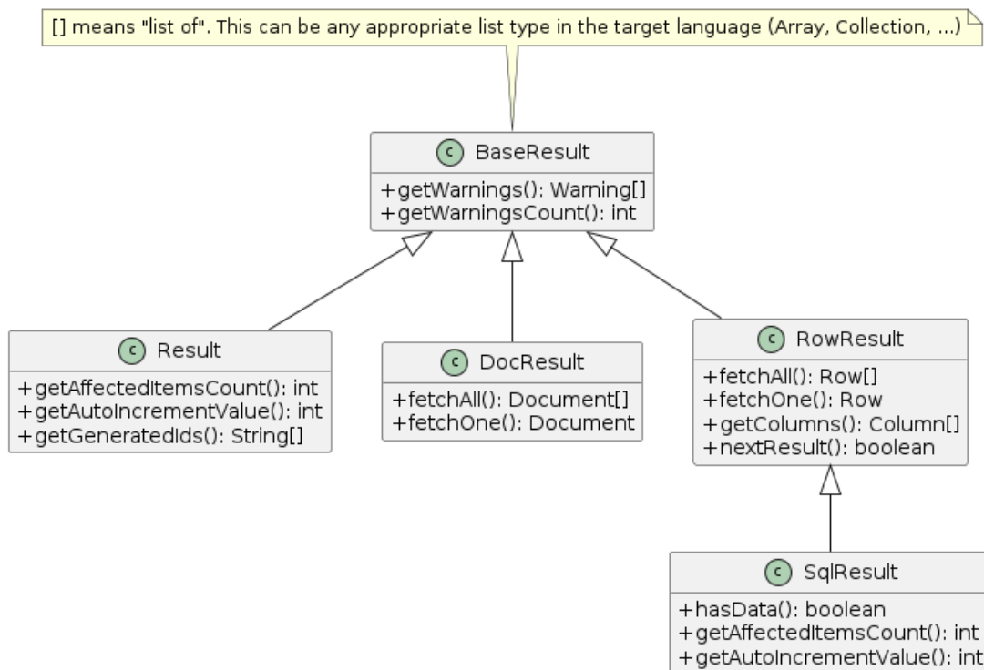
Figure 9.1 Result Classes
